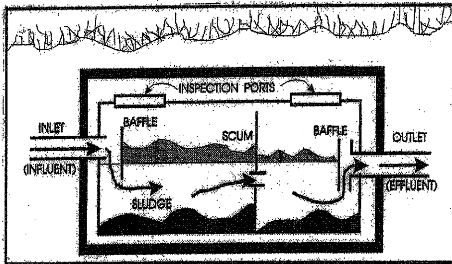
FIGURE D-1: SEPTIC TANK DIAGRAM
