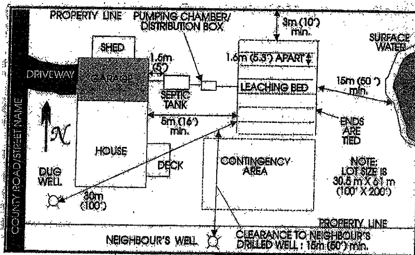
FIGURE G-1: TYPICAL SITE PLAN DRAWING
